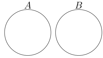
Disjoint Sets
